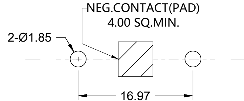
MOUNTING PAD LAYOUT
