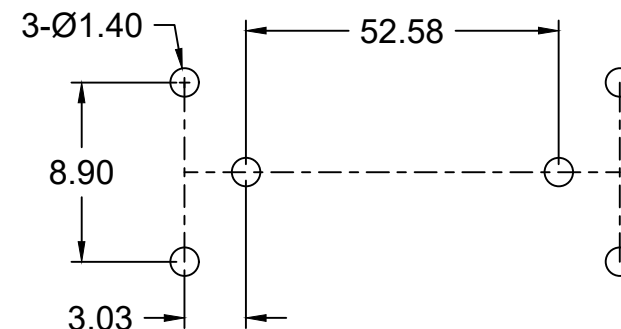
FOR "AA" MOUNTING DETAIL P/N JT-BCKS590S(-) & JT-BCKS596(+)
