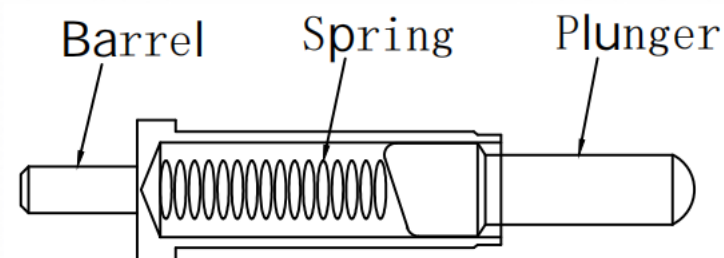
PIN structure
