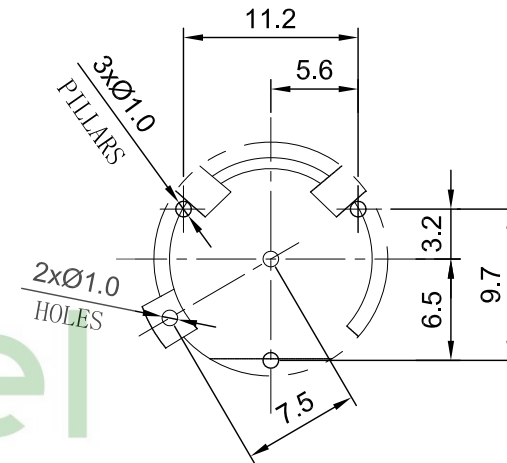
PCB Mounting Layout
