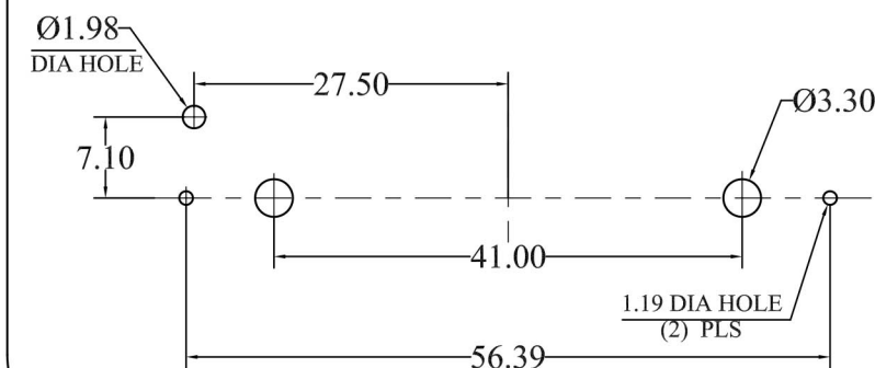
PCB LAYOUT
