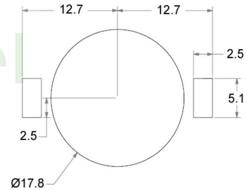
(MOUNTING PAD LAYOUT)
