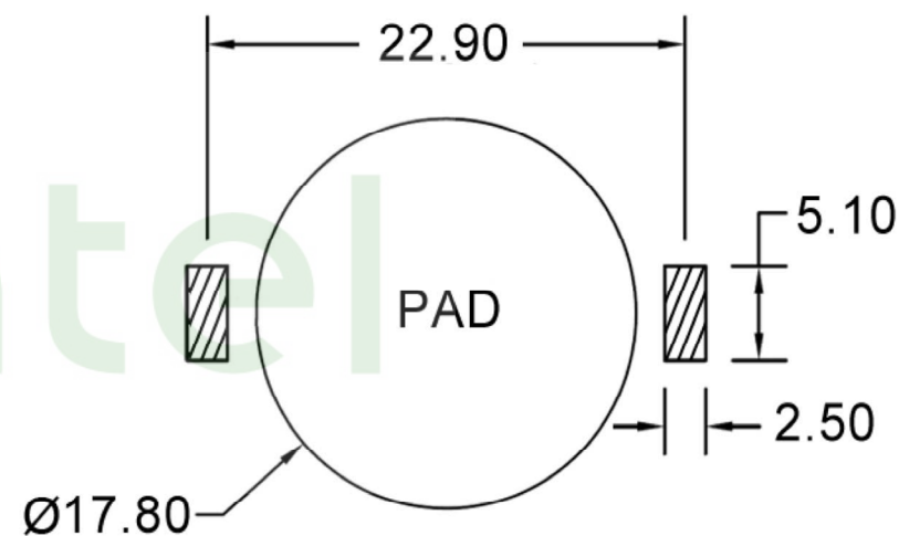
MOUNTING PAD LAYOUT
