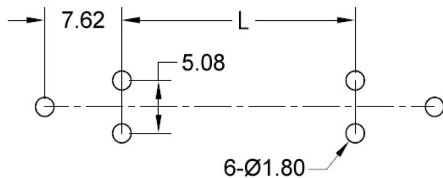
(MOUNTING DETAIL)
