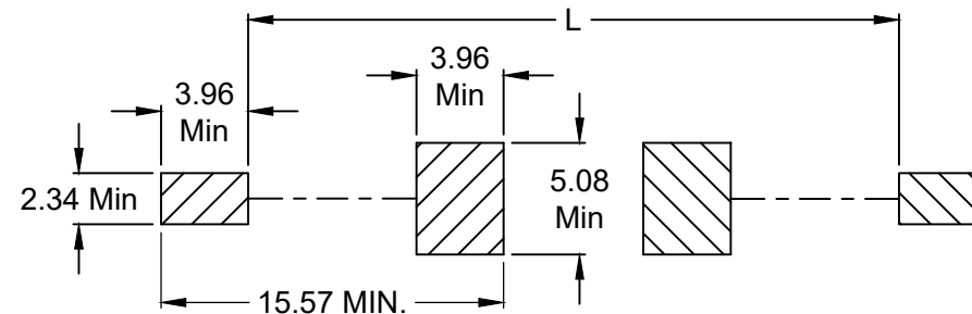
MOUNTING PAD LAYOUT
