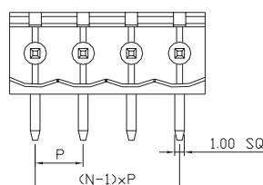
PIN Header(R)
