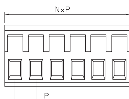
PIN Header(S)
