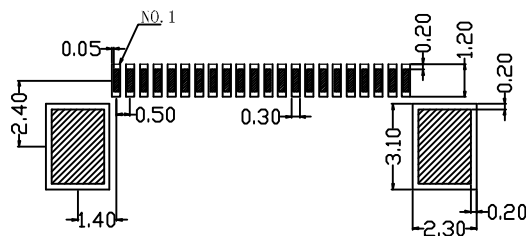
PCB LAYOUT
